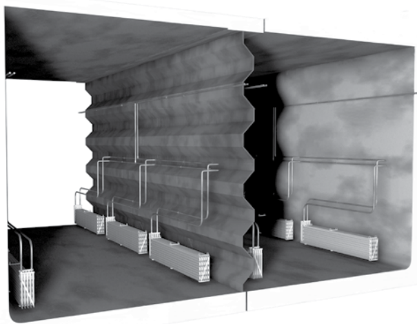
PLATECOIL based cargo heating system in articulated tug barges. Please note the drawing is not to scale; banks and piping are enlarged for clarity.
